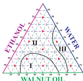
Figure 1. Different types of emulsions in Walnut oil/ Water / Ethanol System.
