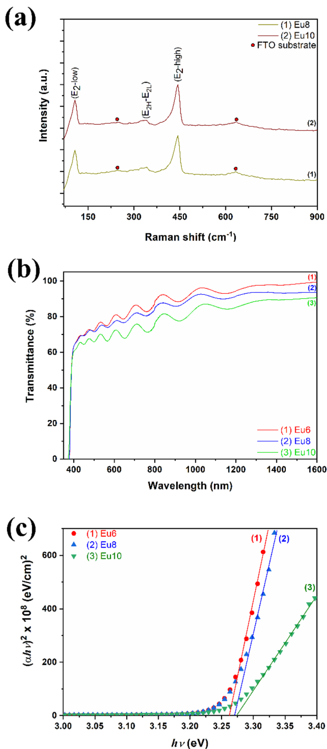
Figure 5. (a) Raman spectra of ZnO:Eu nanowires deposited with different Eu contents: (1) 8 and (2) 10 \mu M. (b) Transmission spectra of ZnO:Eu nanowires with different Eu contents: (1) 6, (2) 8, and (3) 10 \mu M. (c) Plot of (\alpha h\nu)^2 vs (h\nu) for ZnO:Eu nanowires with different Eu contents: (1) 6, (2) 8, and (3) 10 \mu M.
