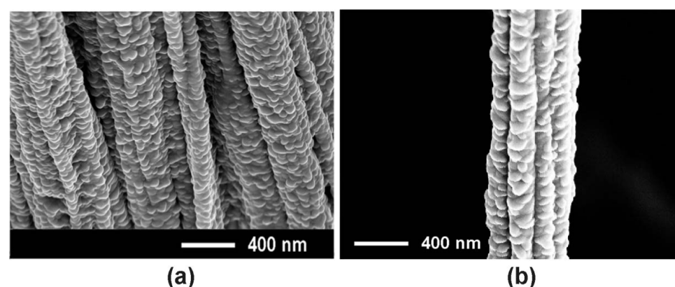
Figure 3. (a) SEM image of a GaAs nanowire array coated with a \text{TiO}_2 layer; (b) SEM image of a GaAs nanowire bundle coated with a \text{ZnO} layer.
