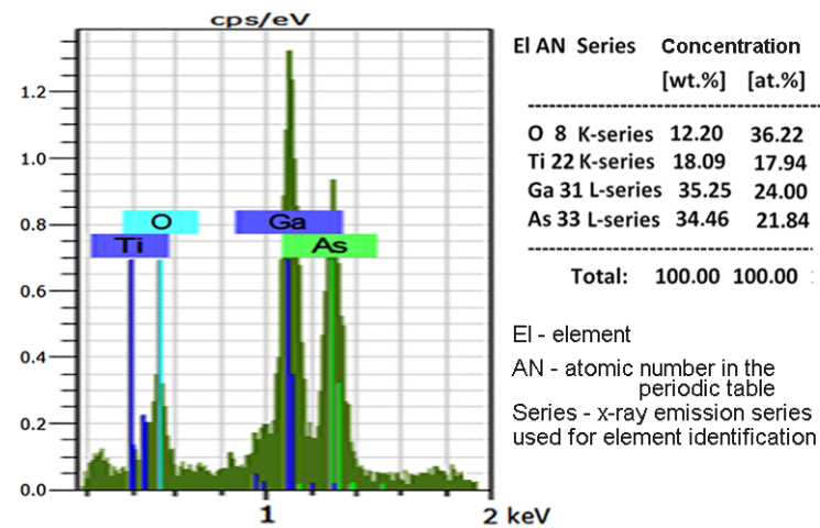
Figure 4. EDX analysis of a GaAs nanowire array coated with TiO 2 by ALD.
